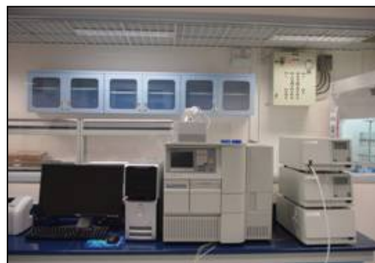
HPLC - Sugars
